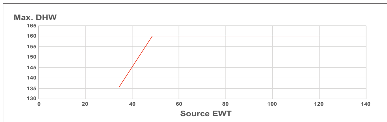
Diagram 1: MHP0270R Maximum Source EWT - Maximum DHW
