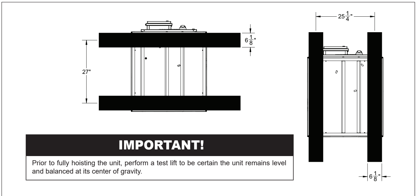
Figure 5: MHP0270R Mounting Rails Positions and Widths
