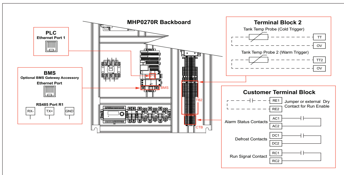
Diagram 5: MHP0270R Control Wiring
