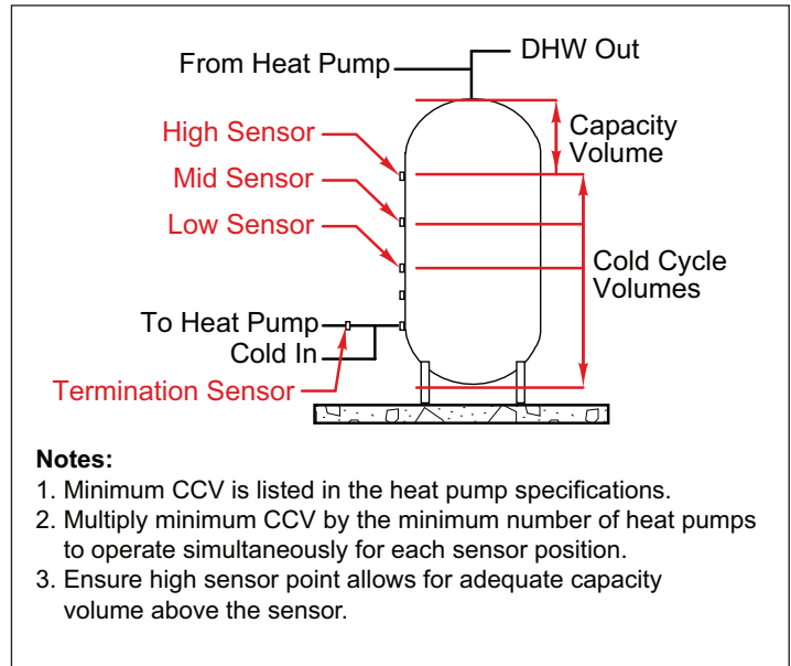
Figure 8: Single-pass, Multiple Heat Pumps with Central Controller
