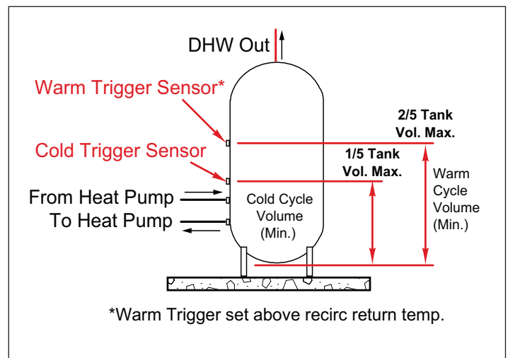
Figure 9: Multi-pass, Single Tank Sensor Locations
