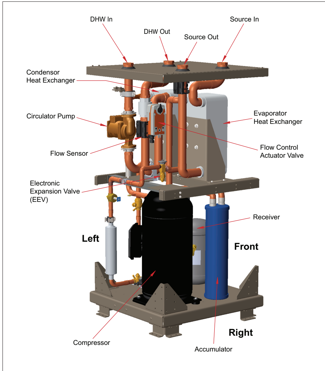
Figure 1: MHP0270R Water Source Heat Pump Water Heater
