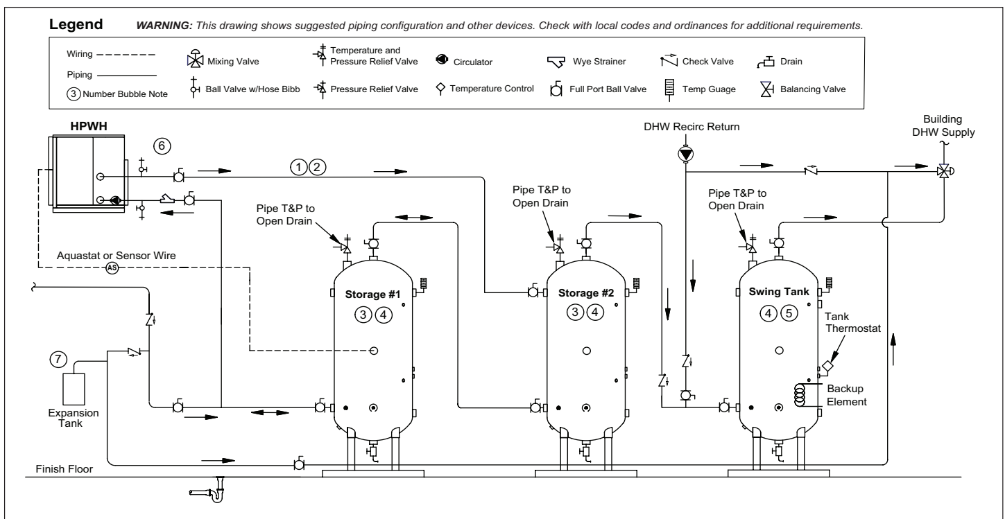
Diagram 2: Single-pass Piping Concept
