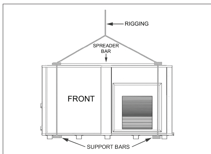
Figure 2: Rigging and Hoisting Unit
