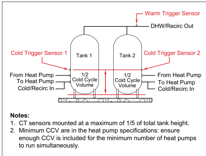
Figure 10: Multi-pass, Multiple Tanks with Central Controller
